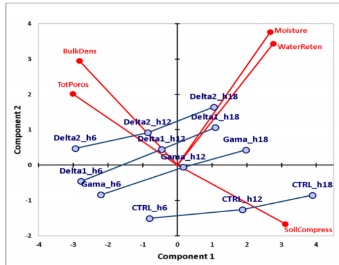
Figure 11. Principal component analysis (PCA) biplot for different depths (factor h) and for the three active elements (factor Device) for soil type S1-S6.
