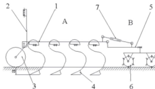
Figure 2. General scheme of a vibro-combinator [2,8,22]
